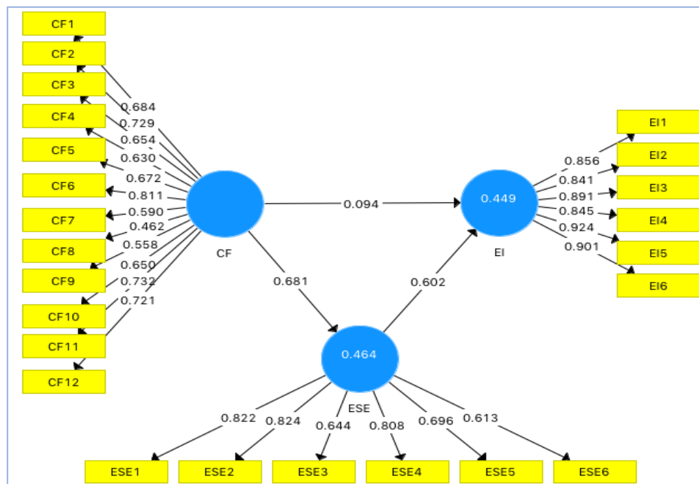
Gambar 2 Model Struktural PLS
