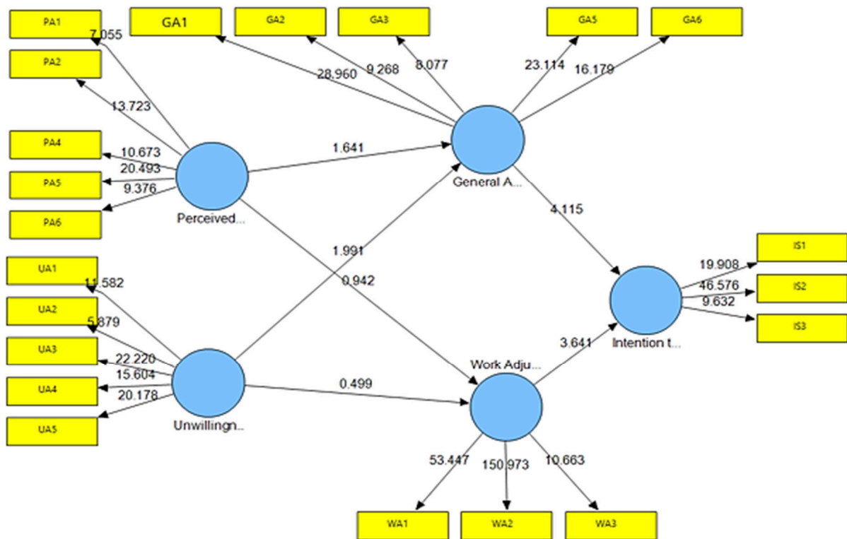
Gambar 2 Path Coefficient
